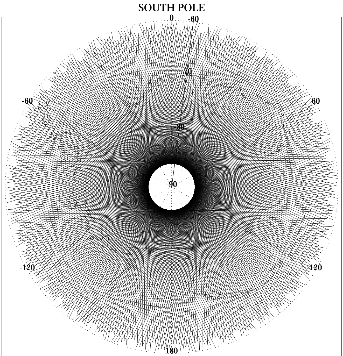
Fig. 3.4 First 25 day near repeat subcycle of 183 day exact repeat ground t rack
