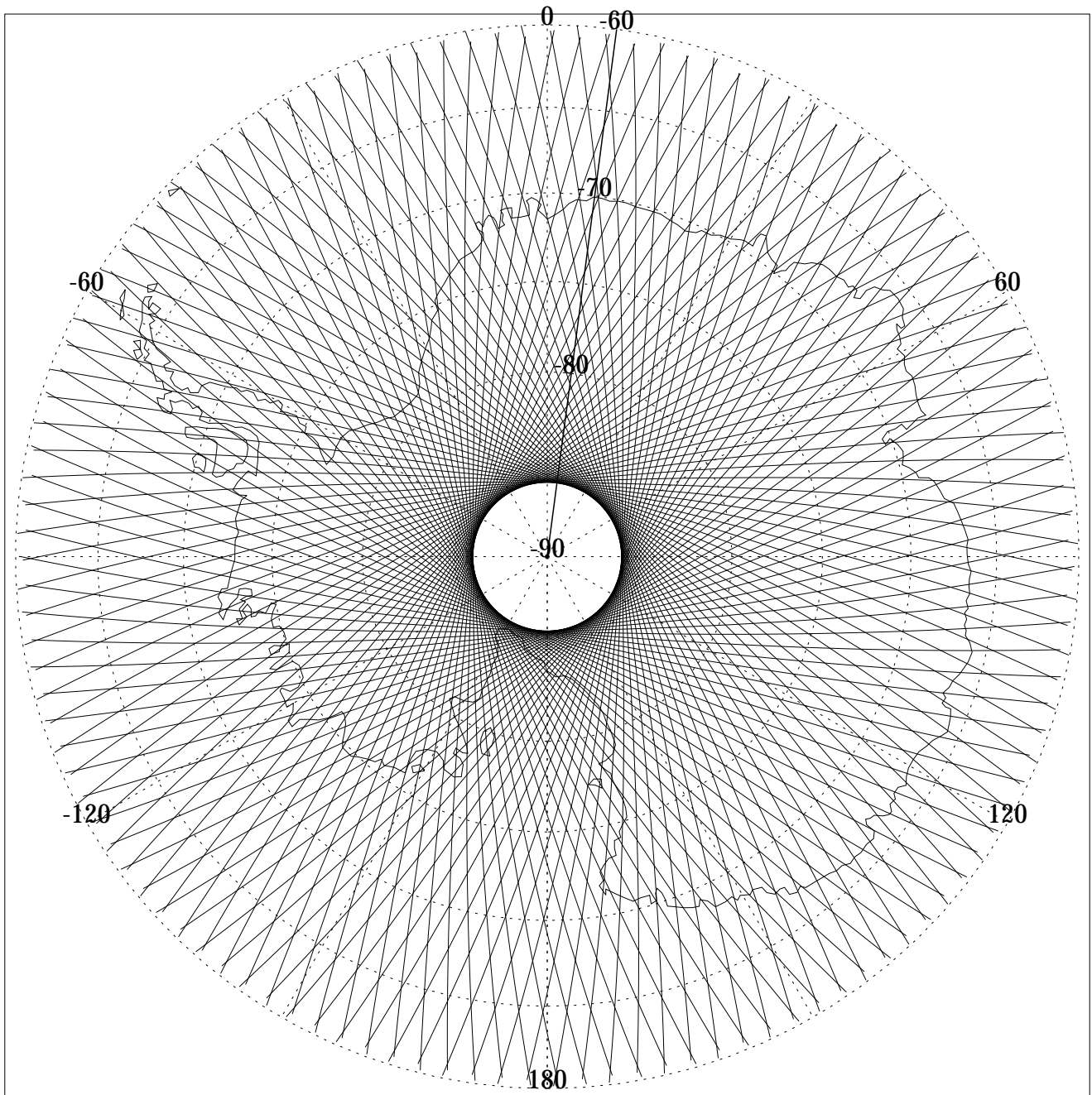
Fig. 3.2 Eight day repeat orbit over Antarctica
